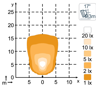
Antares Go 610 1000lm Wide Flood
