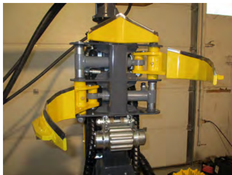
All knives are moving. Measuring wheel with magnetic pick-up.
