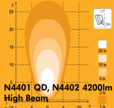
N4401 QD, N4402 4200lm Flood
