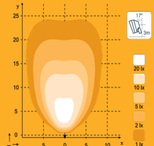
N4401 QD, N4402 3360lm Diffused
