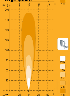
N4403 QD, N4404 3000lm High Beam
