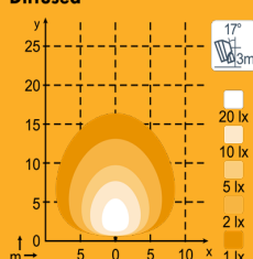
N4403 QD, N4404 2400lm Diffused
