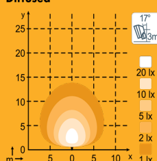
N4405 QD, N4406 1680lm Diffused
