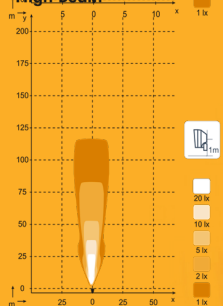
N4405 QD, N4406 2100lm High Beam
