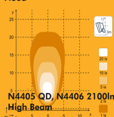
N4405 QD, N4406 2100lm Flood
