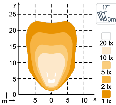
N4403 QD, N4404 3000lm Wide Flood
