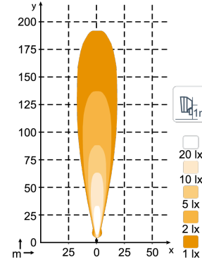
N4403 QD, N4404 3000lm High Beam
