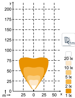
N4403 QD, N4404 3000lm Low Beam
