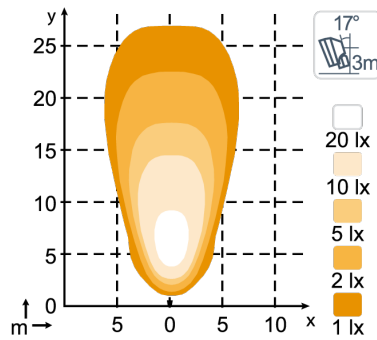
N4403 QD, N4404 3000lm Flood
